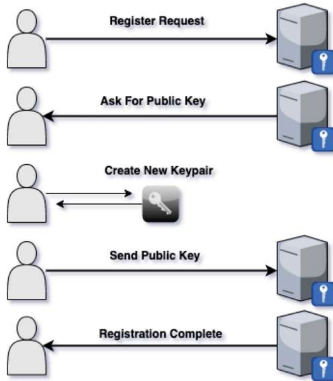
Register Flow
